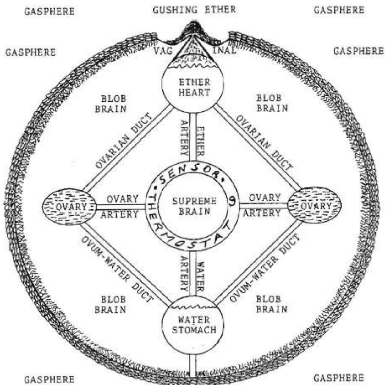
SHAPE NINETEEN HALF SECTION OF A FEMALE SUN (side view)
