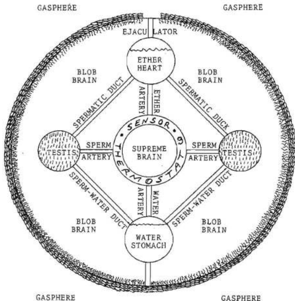
SHAPE EIGHTEEN HALF SECTION OF A MALE SUN (side view)
