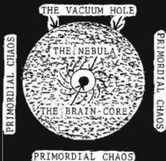
SHAPE NINE MATTER INVASION OF VACUUM HOLE THE ROTATING-GROWING NEBULA
