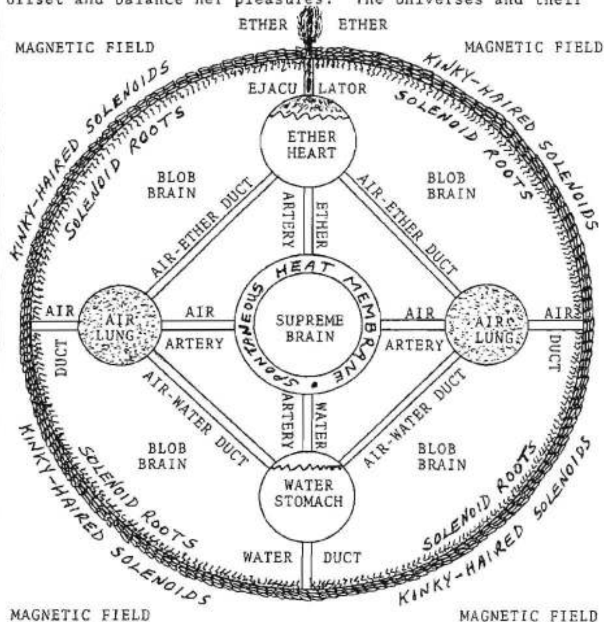
SHAPE SEVENTEEN HALF SECTION OF A MALE SUN (front view)
