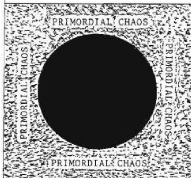
SHAPE EIGHT THE VACUUM BLACK-BALL HOLE THE BEGINNING OF A UNIVERSE
