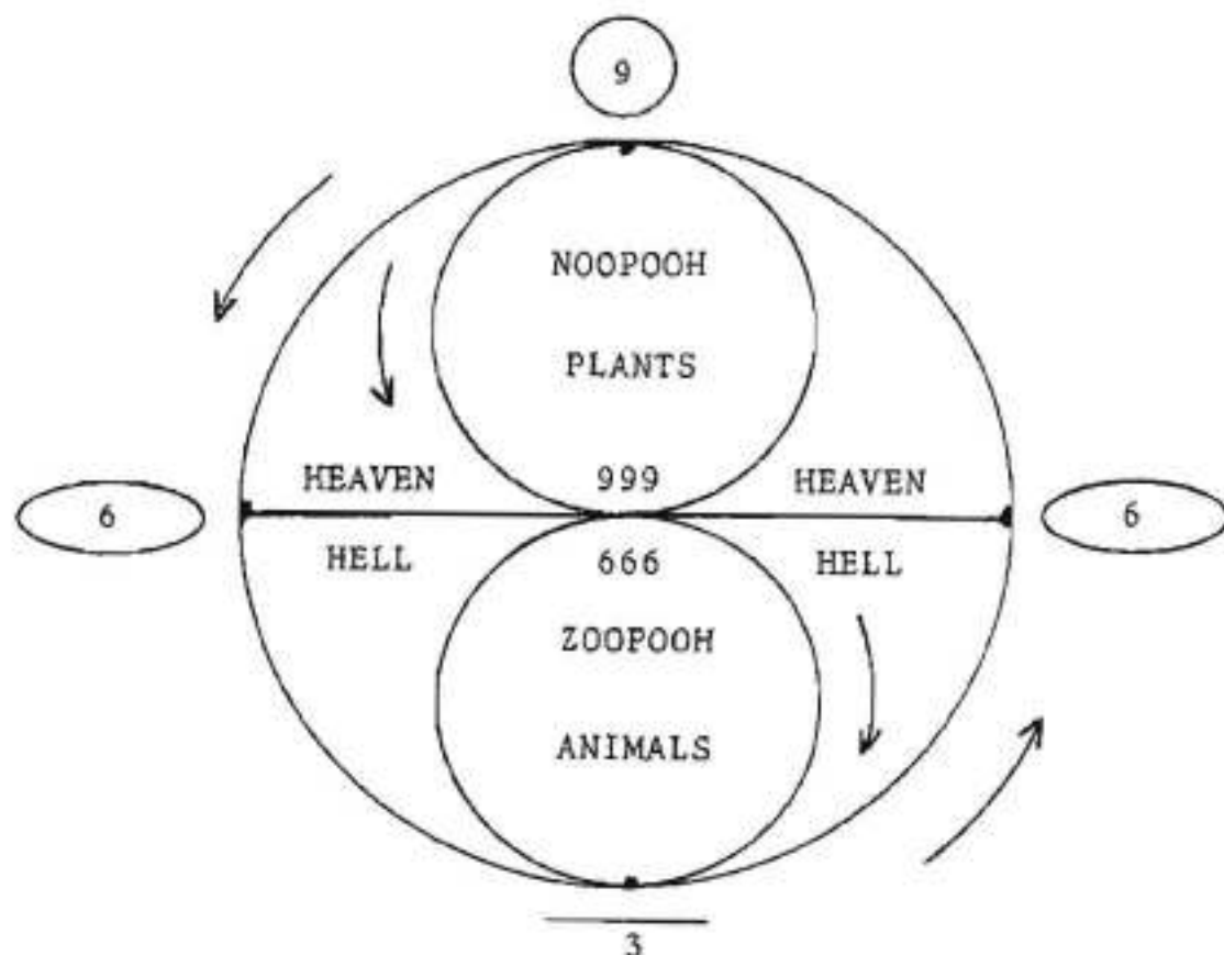
SHAPE FIVE THE GROWTH PATTERN HEAVEN AND PLANTS HELL AND ANIMALS
