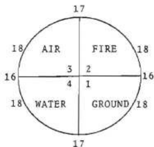
SHAPE FIFTY-ONE THE FORMULA CIRCLE AS THE SMAT CIRCLE OF ORDER EIGHTEEN (18) MAJOR CREATION FORMULAS among the four major
