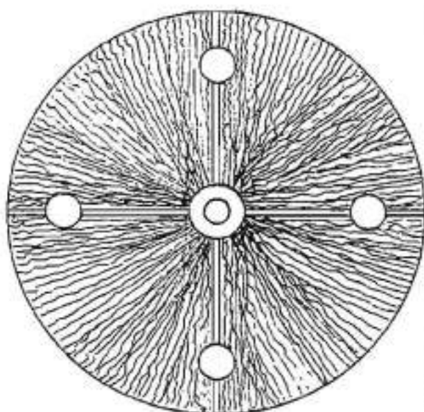
SHAPE TWENTY-THREE A MALE STAR, SHOWING HIS NERVES SYSTEMS
