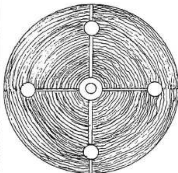
SHAPE TWENTY-TWO A MALE STAR, SHOWING HIS CIRCULATORY SYSTEM
